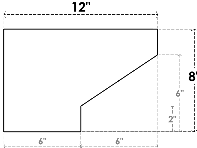
SIDE PROFILE
